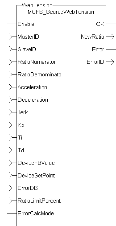
Figure 1-148: MCFB_GearedWebTension Function Block I/O
