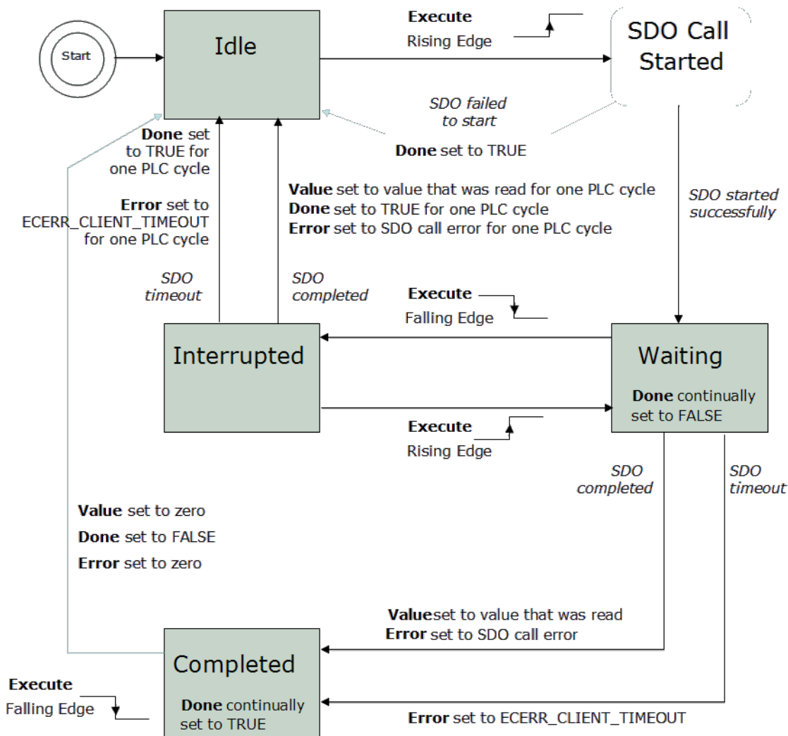
Figure 1-121: ECATReadSdo State Diagram
