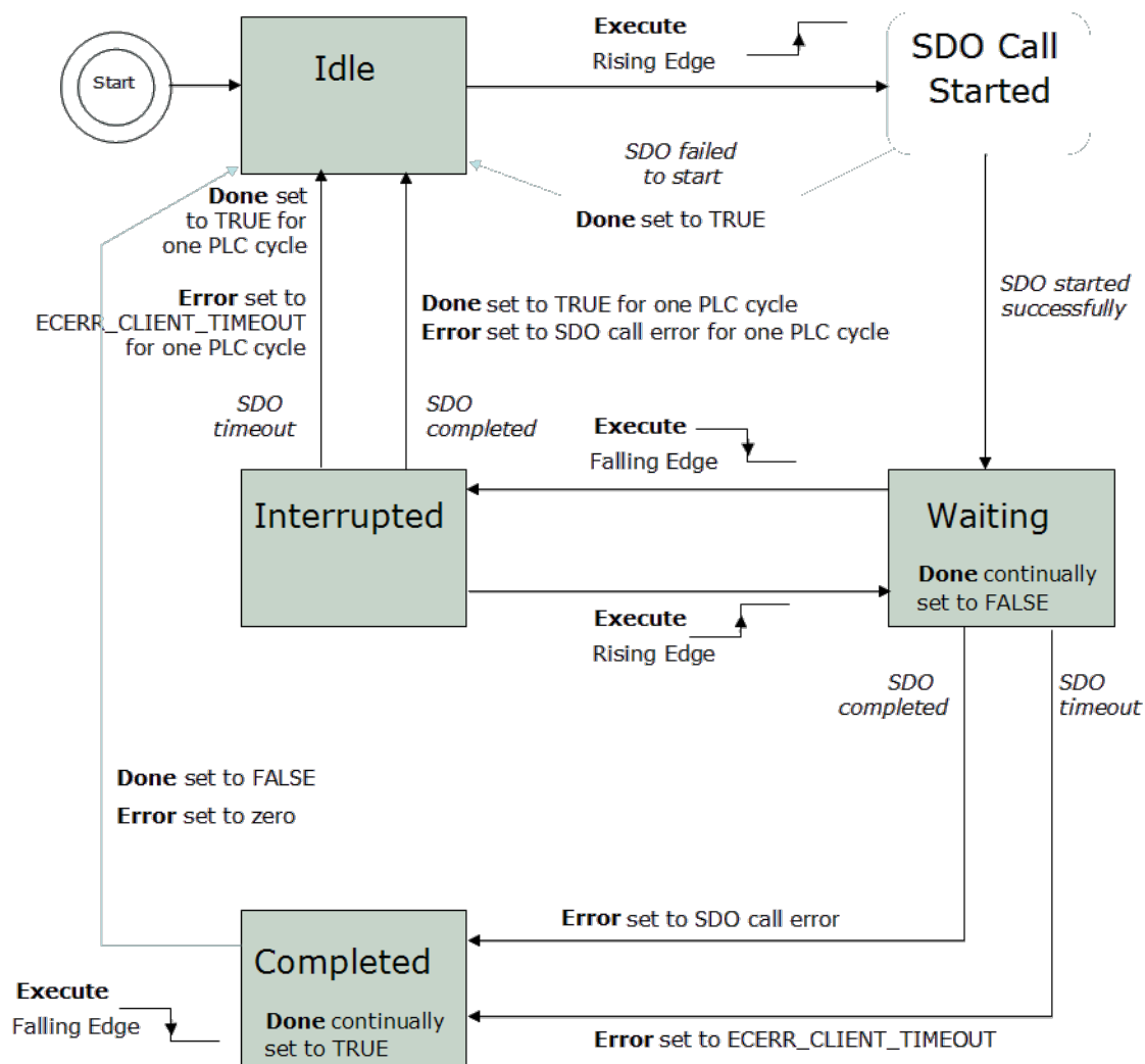
Figure 1-123: ECATWriteSdo State Diagram
