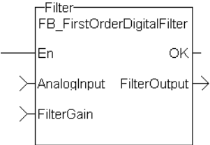
Figure 1-149: CBS First Order Digital Filter
