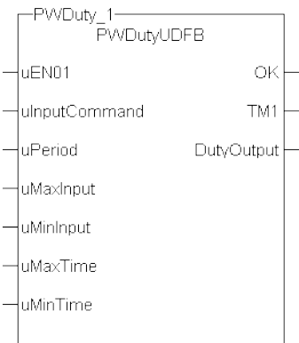
Figure 1-126: Pulse Width Duty Cycle
