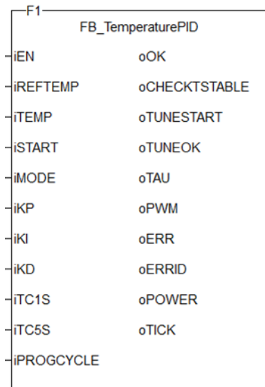
Figure 1-133: The TemperaturePID user-defined function block
